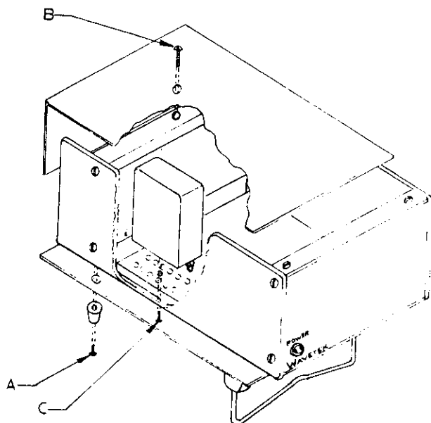
Figure 5-1. Disassembly
