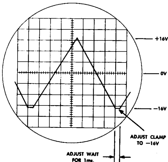
Figure 5-12. Sweep Ramp
