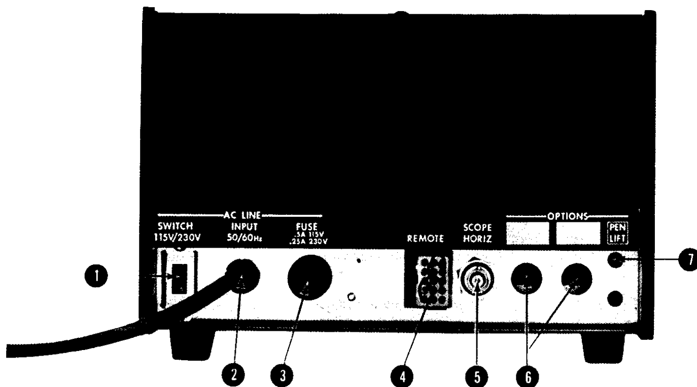
Figure 3-2. Rear Panel
