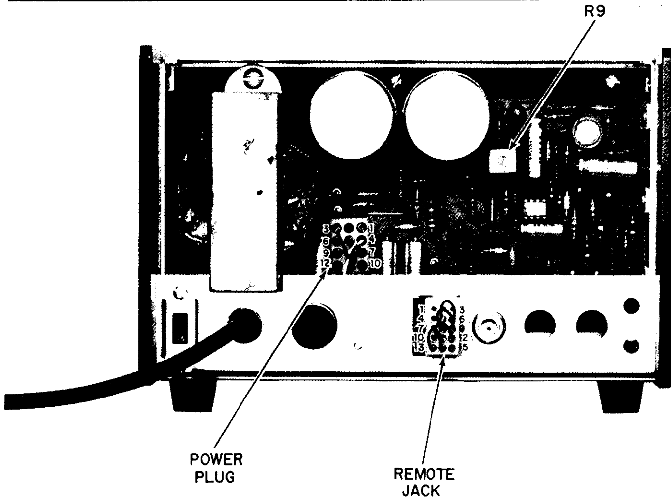
Figure 5-8. Power Supply
