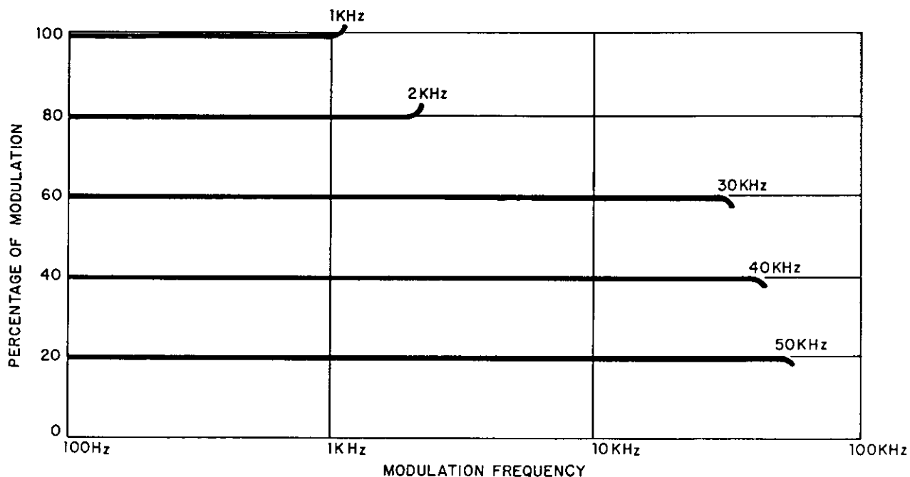
Figure 3-7. Percentage Modulation/Modulating Frequency
