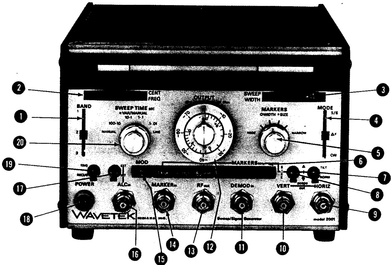
Figure 3-1. Front Panel
