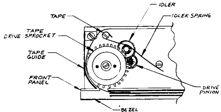
Figure 5-7. Tape Drive
