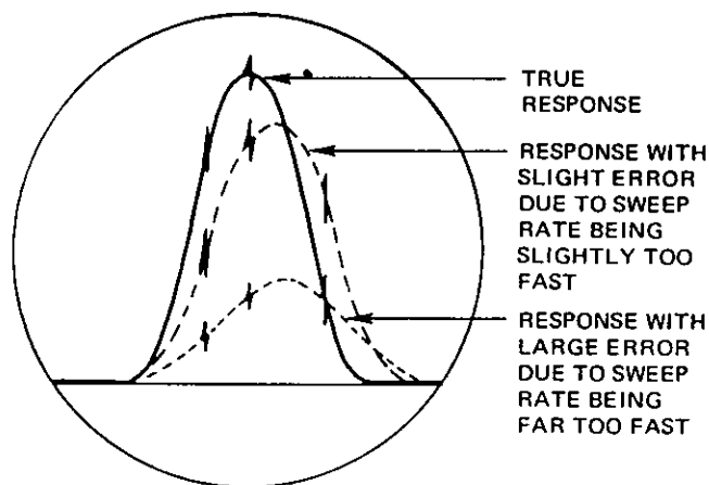
Figure 3-4. Sweep Rate Effects
